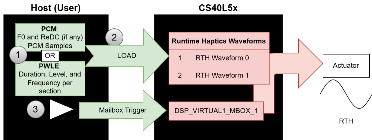
Figure 18 Run-Time Haptics
