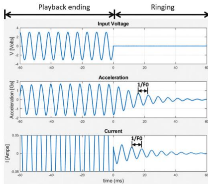
Figure 17 Dynamic F0
