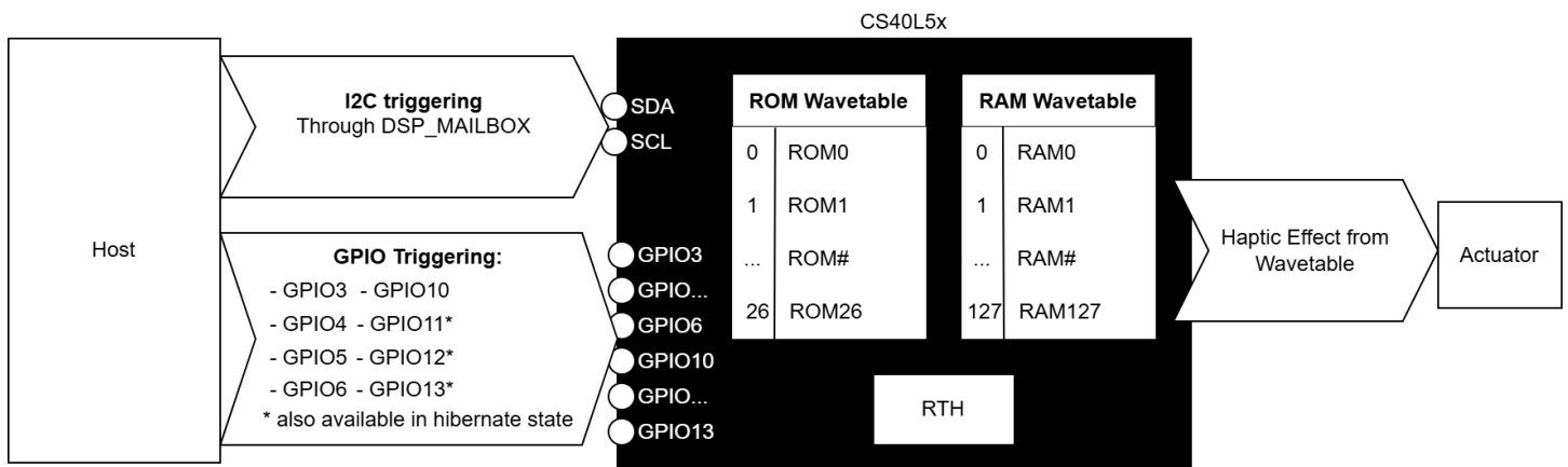
Figure 12 Haptic Playback
