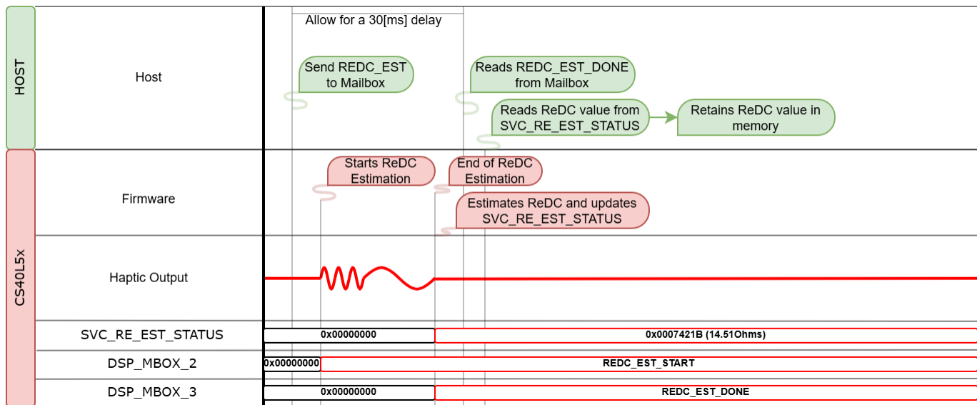
Figure 16 ReDC Calibration
