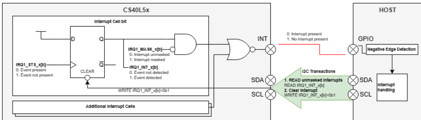
Figure 7 Interrupt Handling
