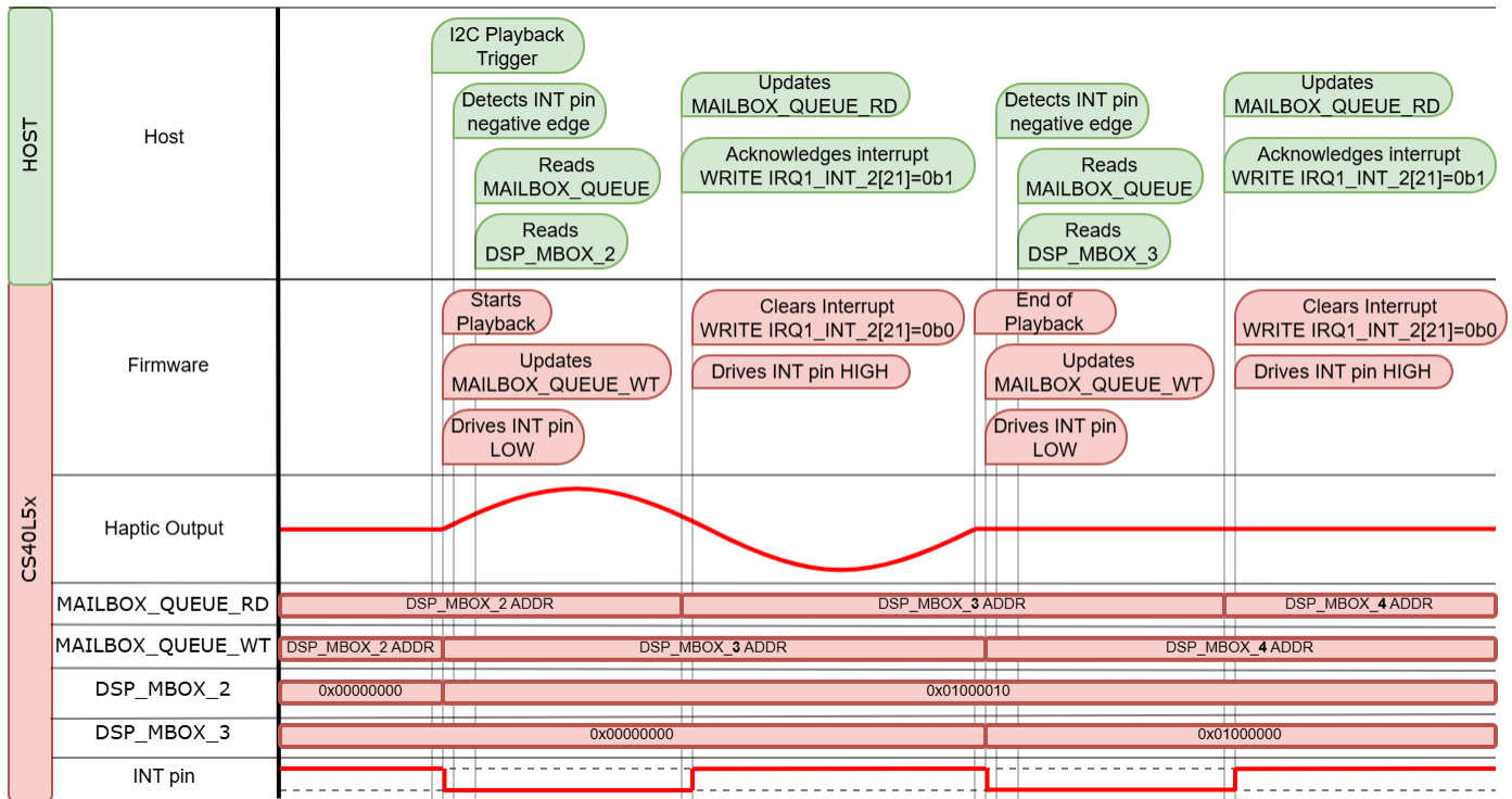
Figure 11 Firmware Interrupt Example
