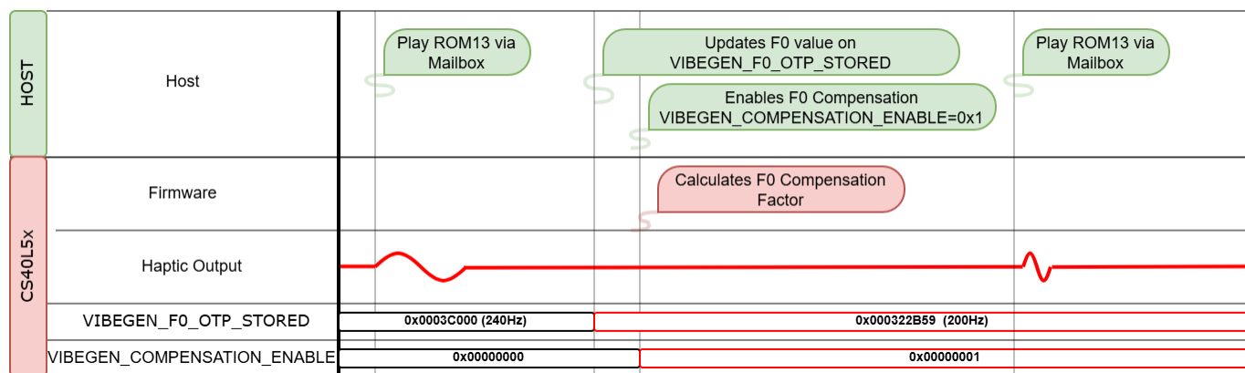
Figure 15 F0 Compensation from User-Defined F0
