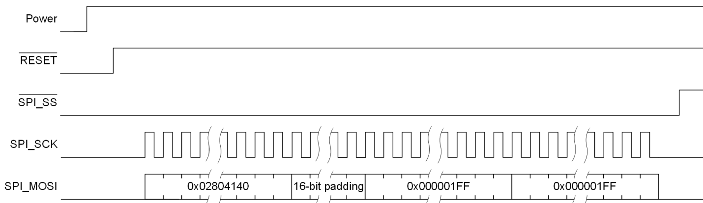
Figure 13 Disable GPIO10 Default Haptic Trigger
