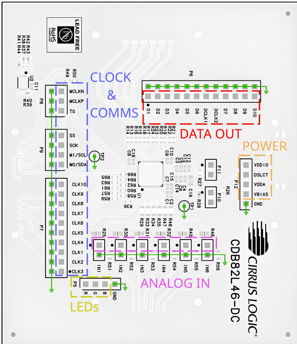
Figure 3. Test Points
