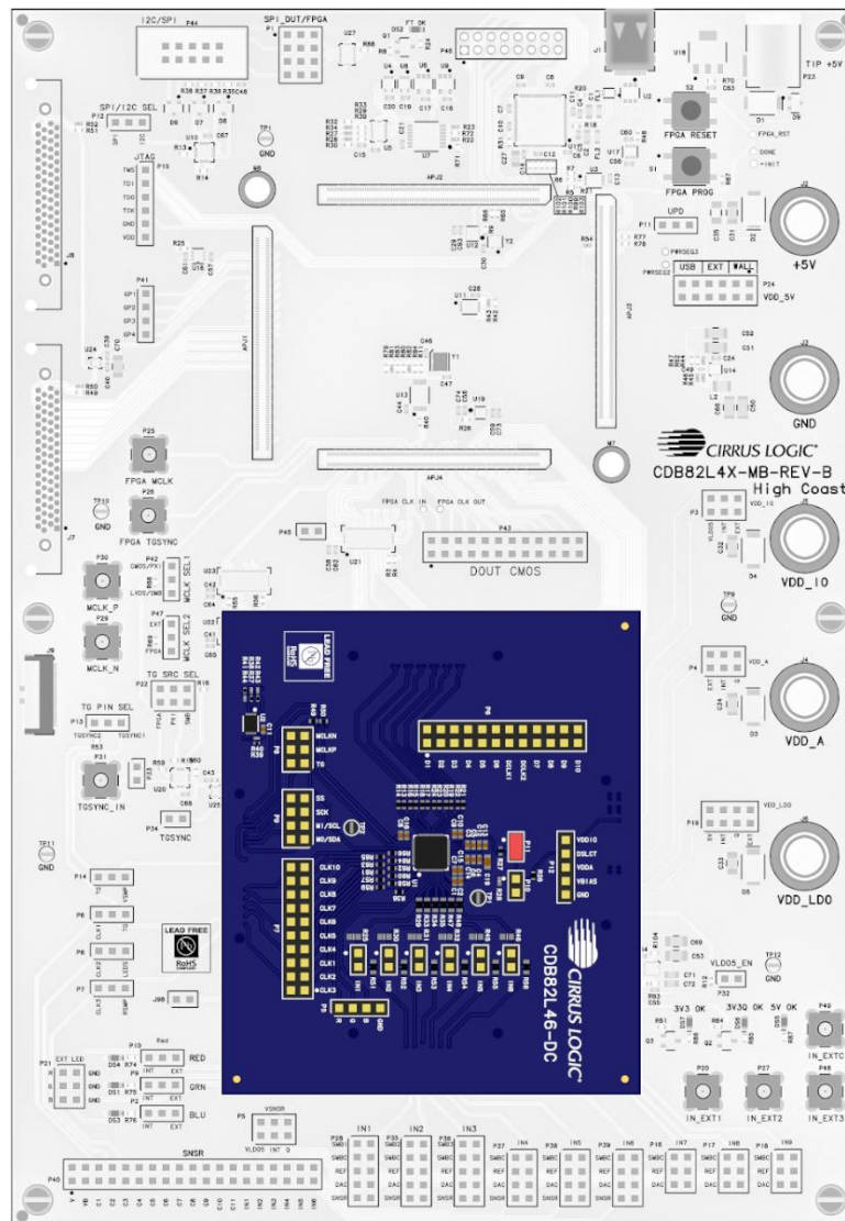
Figure 2. Motherboard Connection
