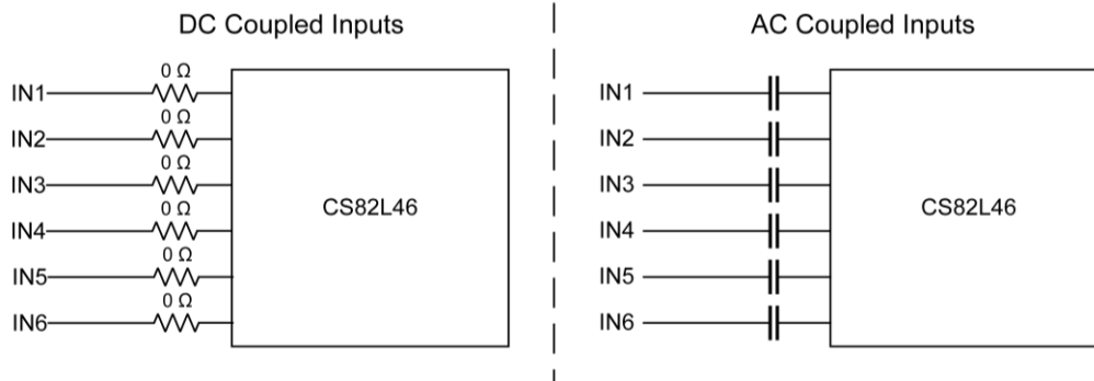
Figure 5. DC/AC Coupled Inputs
