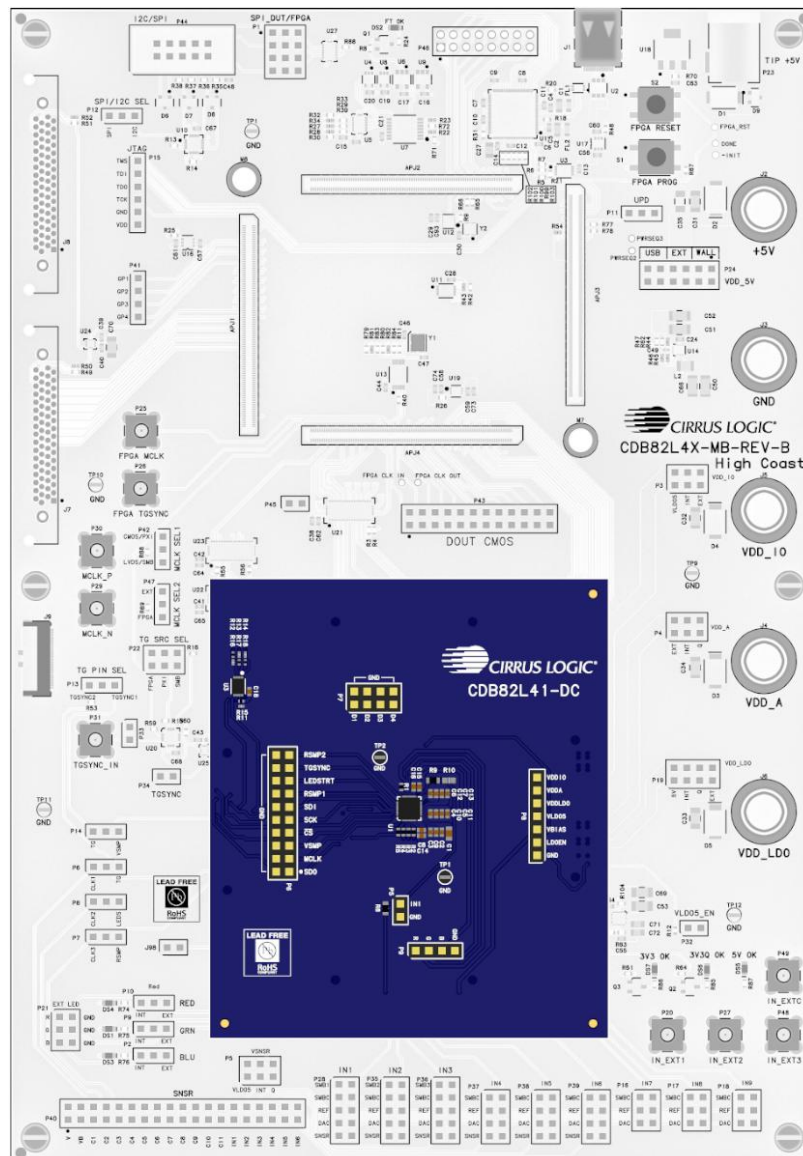
Figure 2. Motherboard Connection
