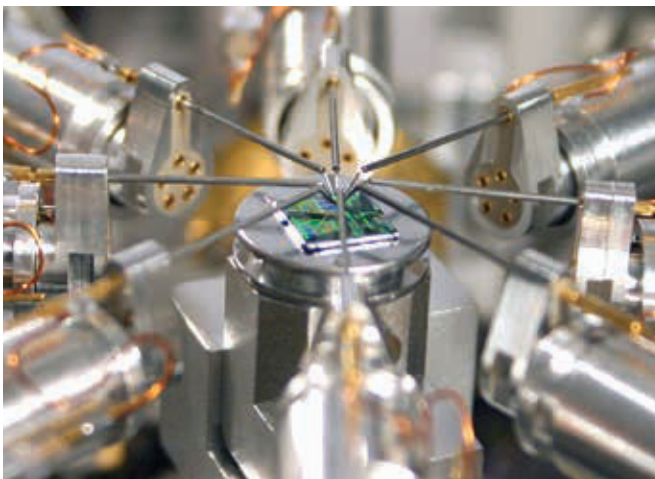
Nanoprobe
