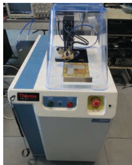
CDM tester
