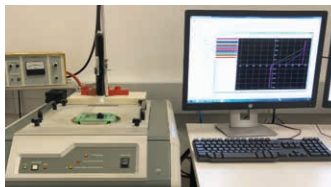
Latch-up tester
