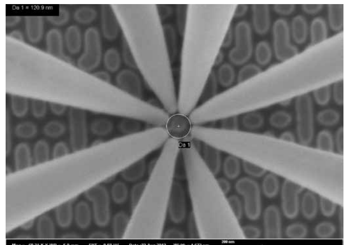
Nanoprobe
