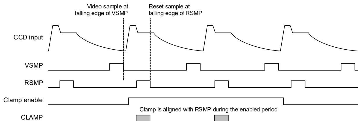
Figure 4-9. Clamp Timing (CDS Mode)
