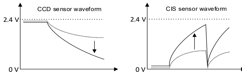
Figure 4-13. Analog Gain
