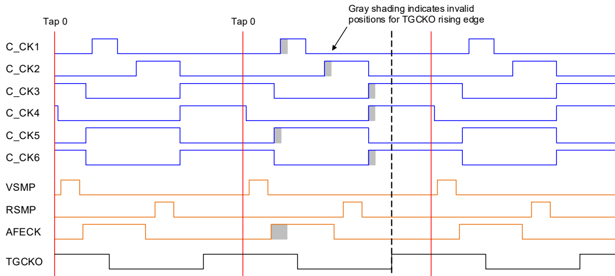
Figure 4-65. Example Clocking Configuration
