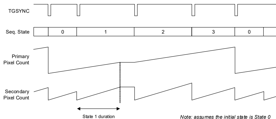
Figure 4-50. TG Slave Mode—Single Cycle, TGSYNC Trigger
