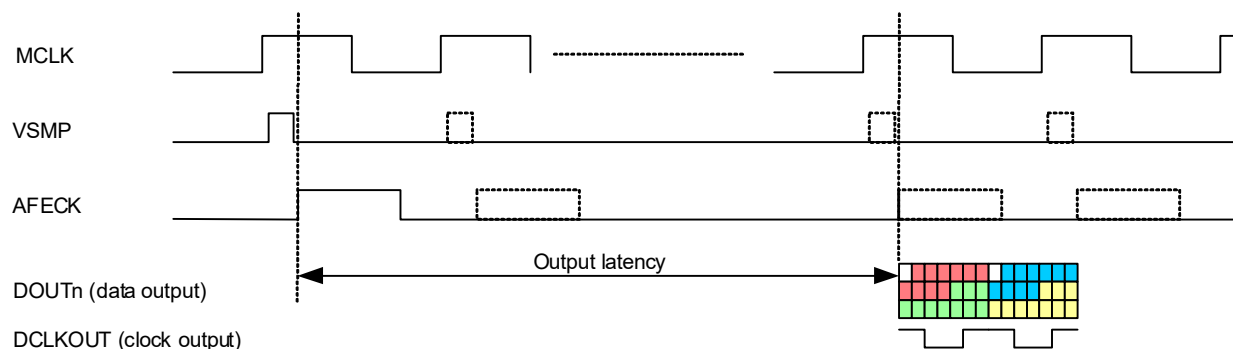
Figure 4-40. Data Output Timing (TG Mode, LVDS Output)
