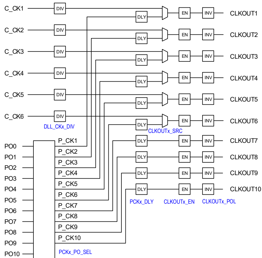
Figure 4-64. Clock Output Configuration
