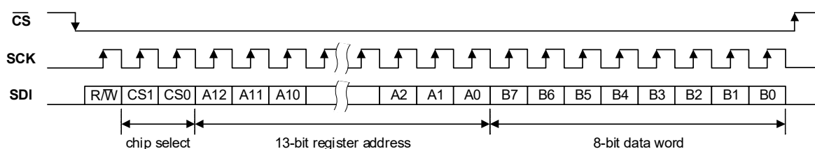
Figure 4-73. Control Interface SPI Register Write—Flat Mode
