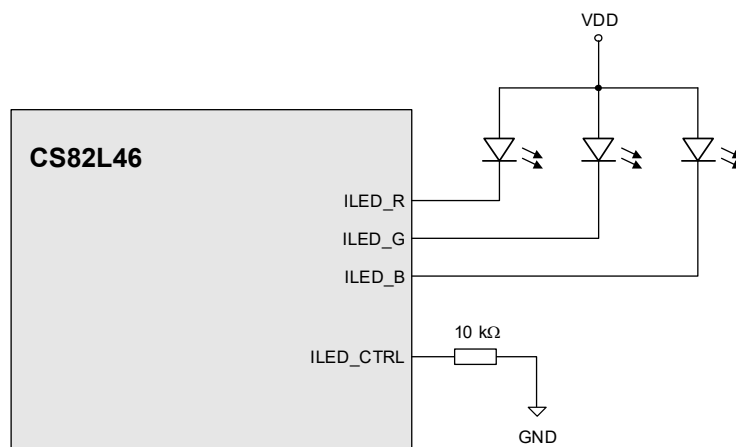
Figure 4-66. LED Output Drivers
