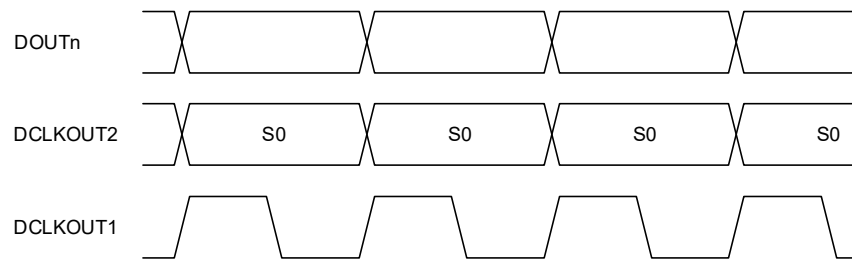
Figure 4-32. CMOS (TG) Output Format
