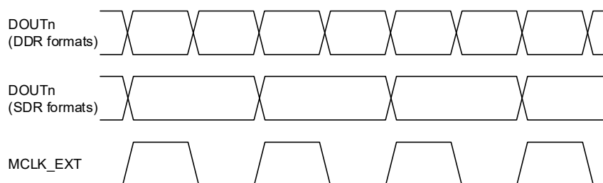
Figure 4-33. CMOS (External) Output Format
