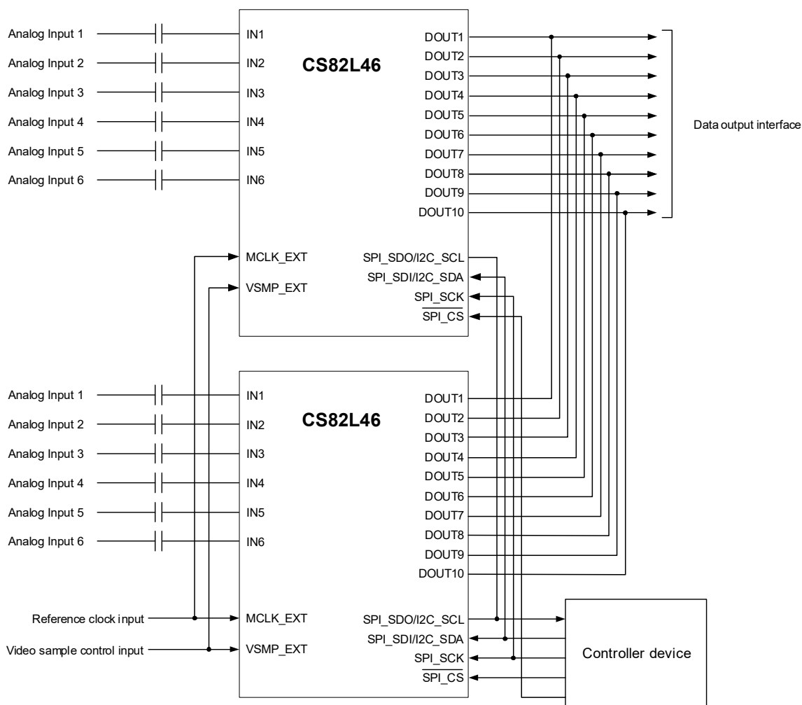
Figure 4-34. TDM Mode
