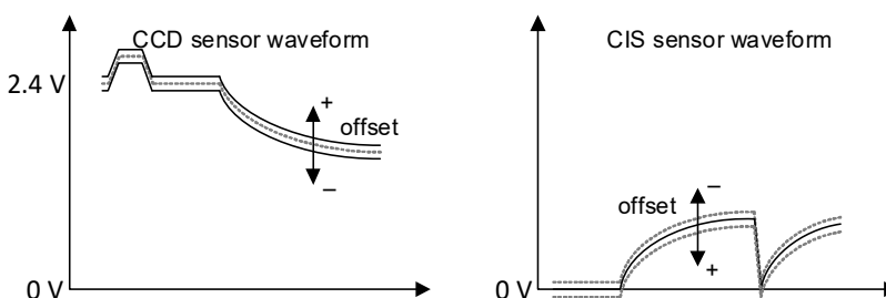
Figure 4-12. Offset Control
