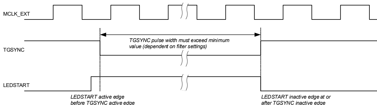
Figure 4-53. TGSYNC/LEDSTART Timing—External Mode
