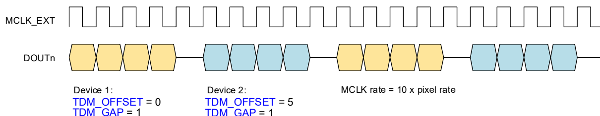
Figure 4-36. TDM Data Timing—Gap Enabled
