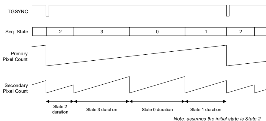
Figure 4-47. TG Master Mode—Multiple States
