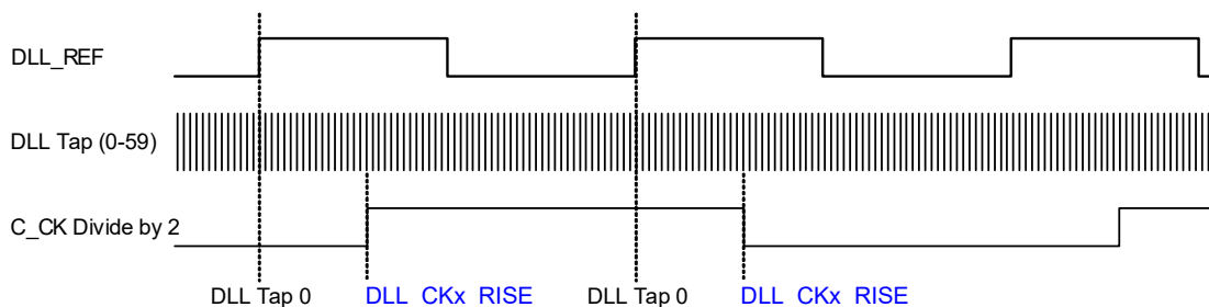
Figure 4-62. Clock Division
