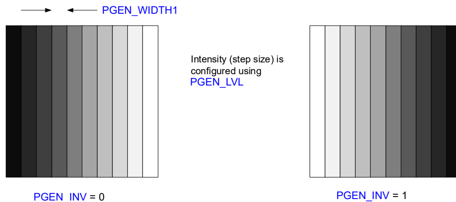
Figure 4-20. Horizontal Ramp
