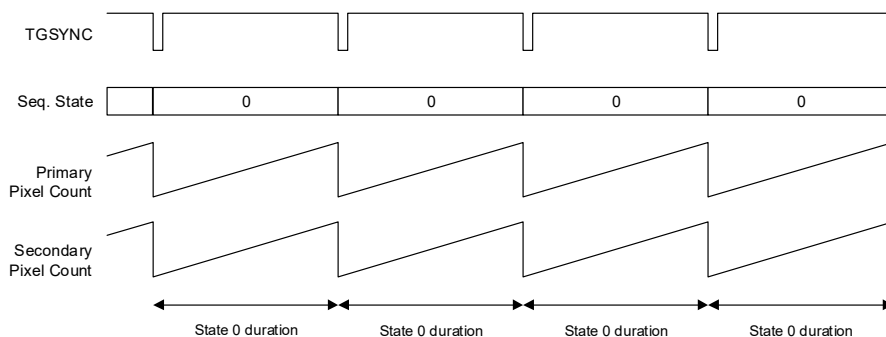
Figure 4-46. TG Master Mode—Single State
