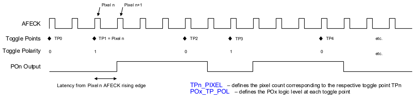
Figure 4-54. Pulse-Output (POn) Configuration—Toggle Point Control
