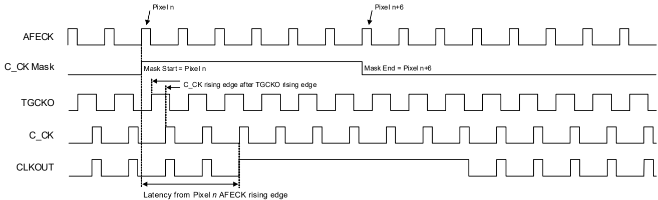
Figure 4-61. Clock Mask Timing—C_CK after TGCKO
