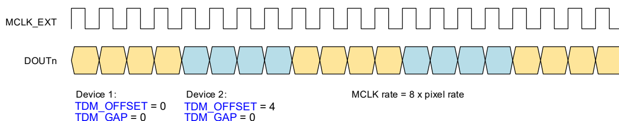
Figure 4-35. TDM Data Timing—Gap Disabled
