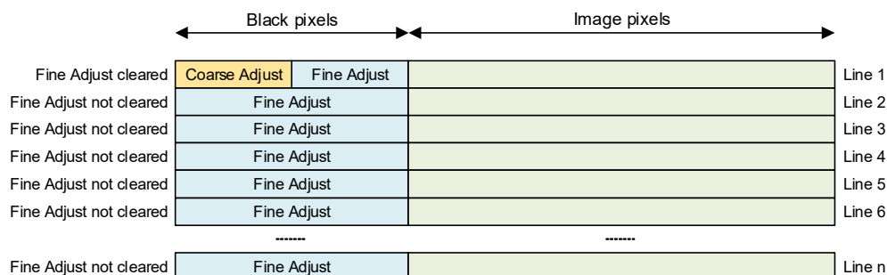
Figure 4-18. Black Level Calibration—Example 3
