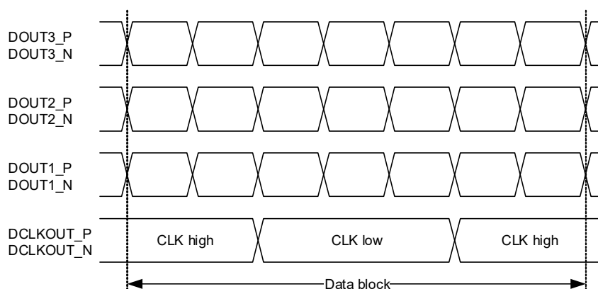
Figure 4-23. LVDS Output Format
