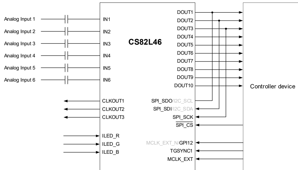
Figure 4-77. Shared Bus Mode
