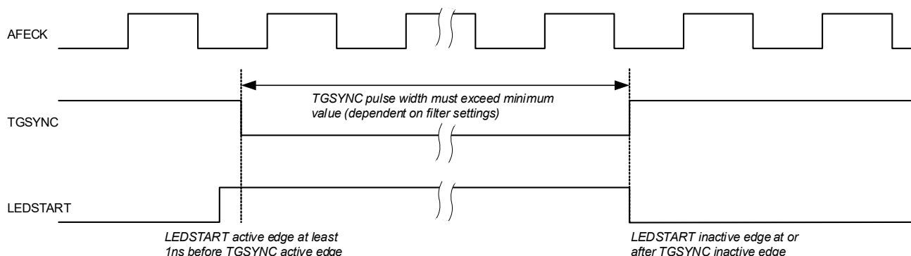
Figure 4-52. TGSYNC/LEDSTART Timing—TG Mode
