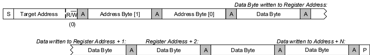
Figure 4-71. Multiple-Register Write to Specified Address
