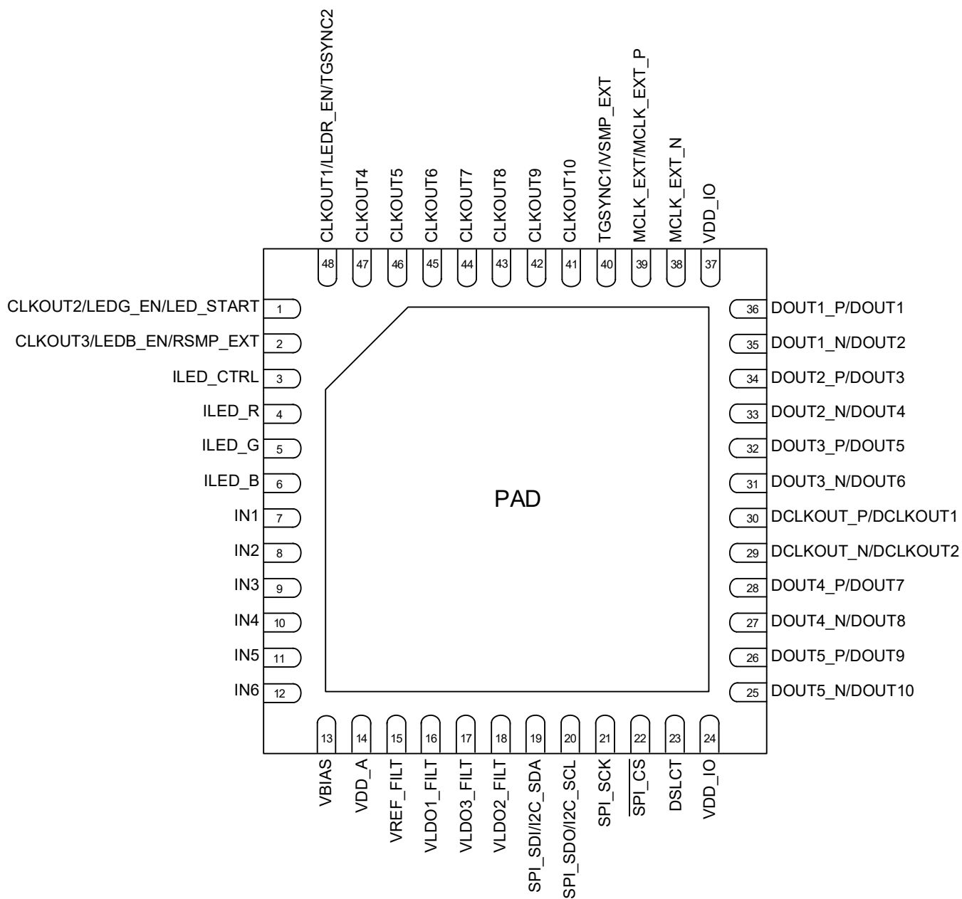
Figure 1-1. QFN 48-pin diagram (Top View, Through Package)
