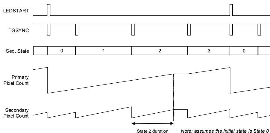
Figure 4-51. TG Slave Mode—Single Cycle, LEDSTART + TGSYNC Trigger
