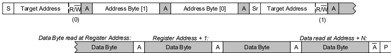
Figure 4-72. Multiple-Register Read from Specified Address
