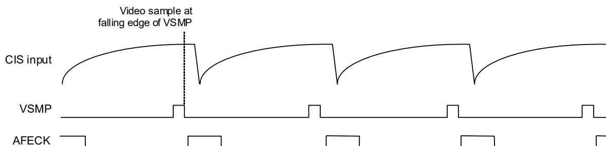
Figure 4-38. Sample Timing Control (non-CDS Mode)
