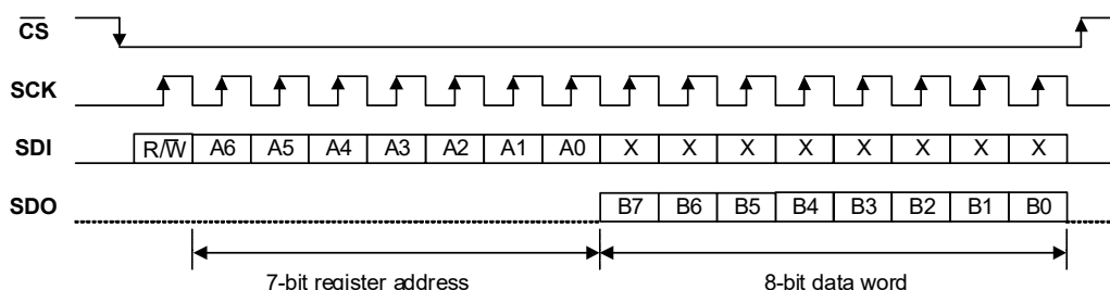
Figure 4-76. Control Interface SPI Register Read—Banked Mode
