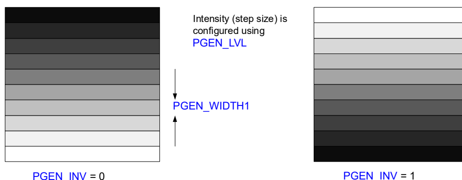
Figure 4-19. Vertical Ramp
