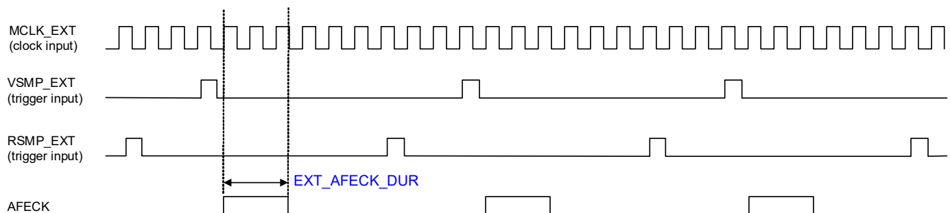
Figure 4-42. Direct-Pin Timing (External Mode 1)
