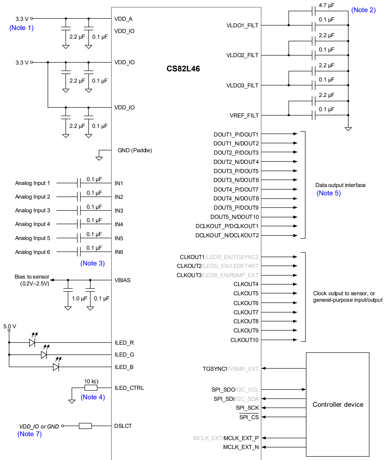
Figure 2-1. Typical Connections—TG Mode
