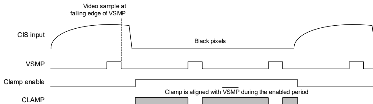
Figure 4-10. Clamp Timing (Non-CDS Mode)
