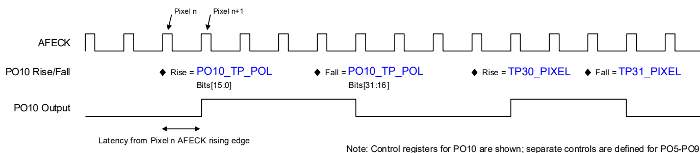
Figure 4-55. Pulse-Output (POn) Configuration—Direct Control
