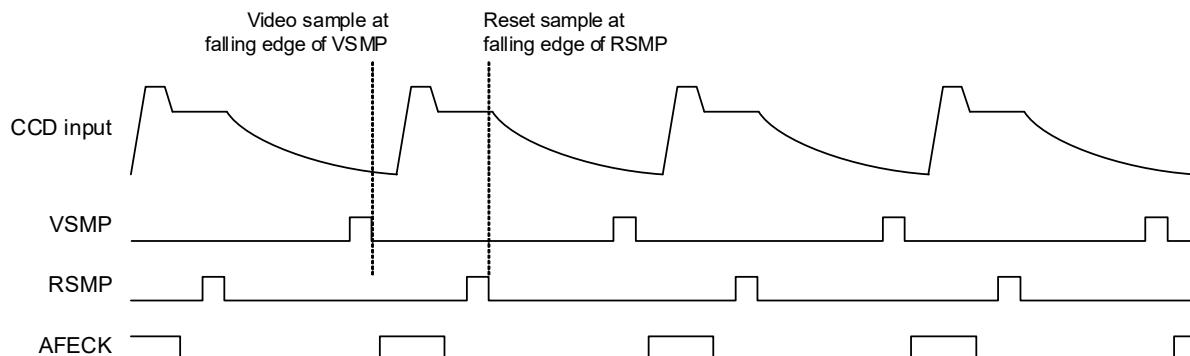
Figure 4-37. Sample Timing Control (CDS Mode)
