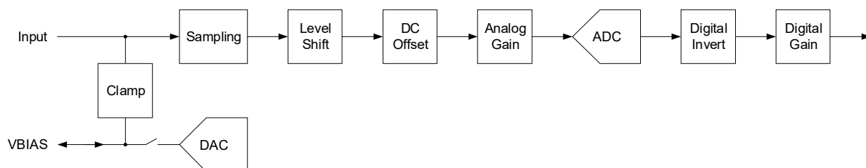
Figure 4-6. Analog Input Path
