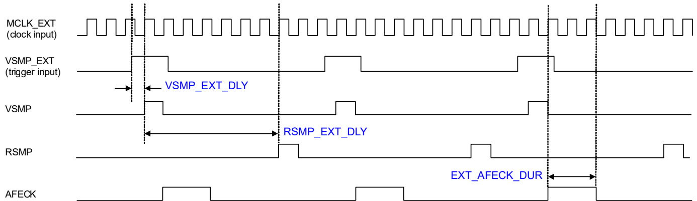
Figure 4-44. MCLK-Aligned Timing Control (External Mode 2)
