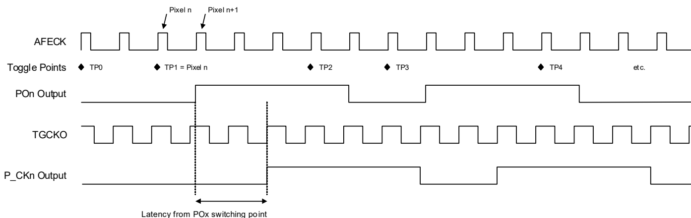
Figure 4-56. Pulse Clock (P_CK) Configuration
