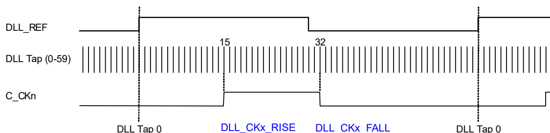
Figure 4-58. High-Speed Clocks (C_CKn)
