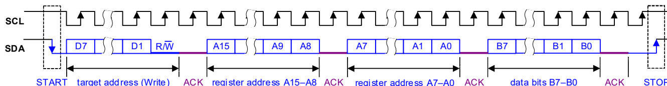
Figure 4-67. Control Interface I 2 C Register Write
