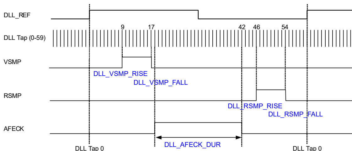
Figure 4-39. DLL Timing Control (TG Mode)
