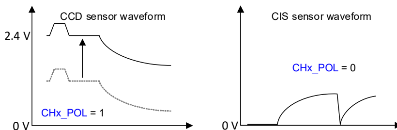
Figure 4-11. Polarity Select
