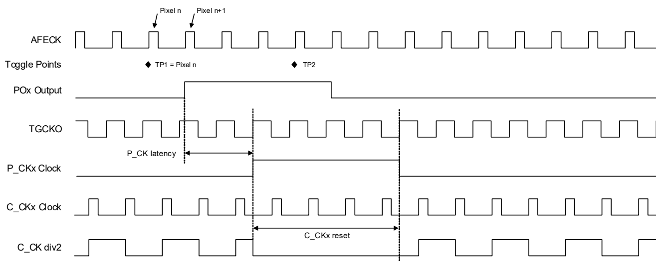
Figure 4-63. Clock Divider Phase Control
