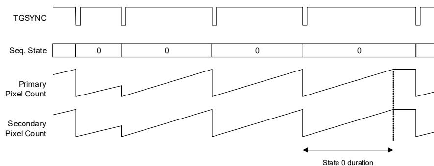
Figure 4-48. TG Slave Mode—Single State
