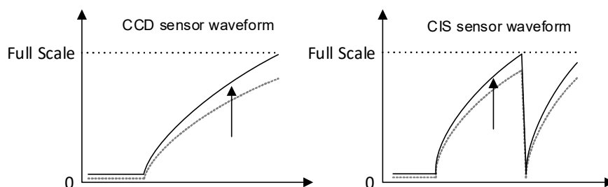
Figure 4-15. Digital Gain
