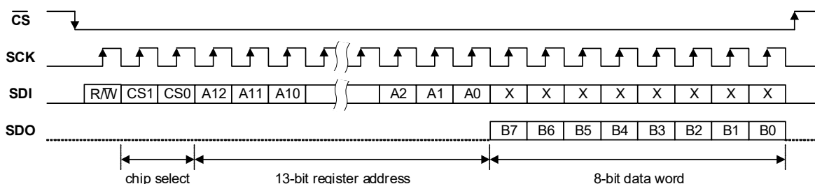
Figure 4-74. Control Interface SPI Register Read—Flat Mode
