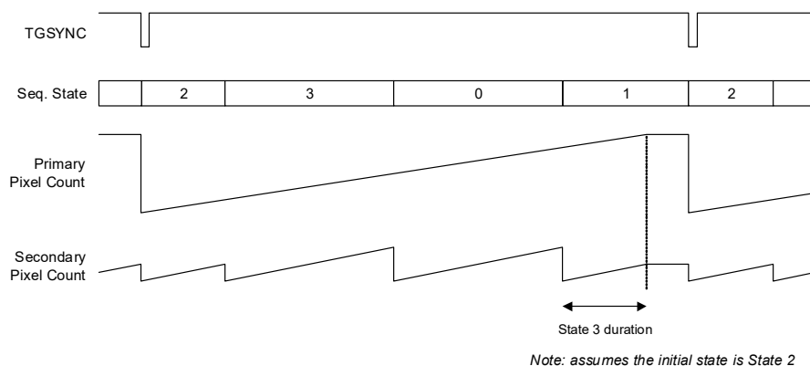
Figure 4-49. TG Slave Mode—Multiple Cycle, TGSYNC Trigger
