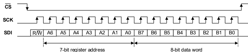
Figure 4-75. Control Interface SPI Register Write—Banked Mode
