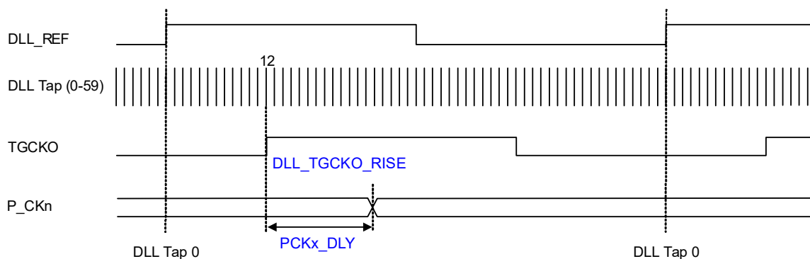
Figure 4-57. Pulse-Clock Switch Timing
