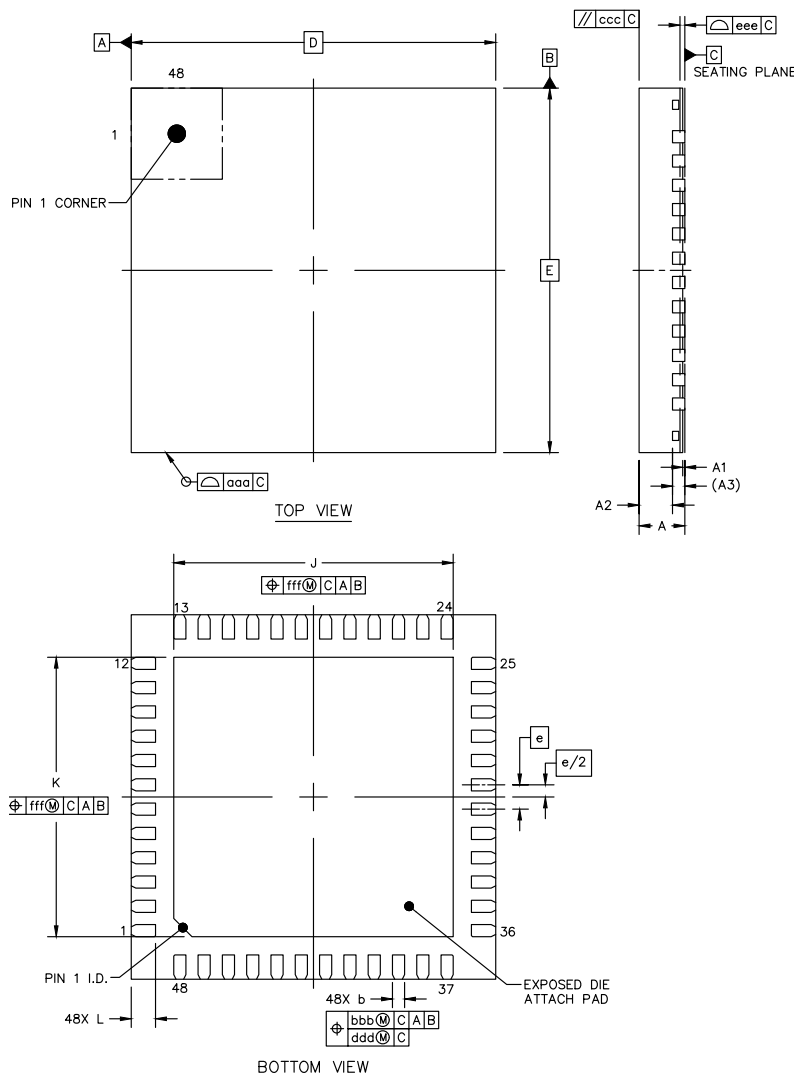
Figure 10-1. QFN 48-pin Package Drawing
