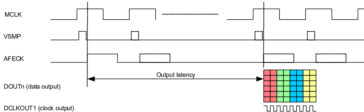
Figure 4-41. Data Output Timing (TG Mode, CMOS Output)
