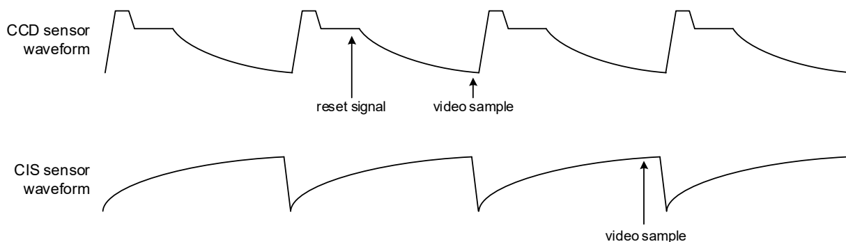
Figure 4-7. Typical CIS/CCD Waveforms
