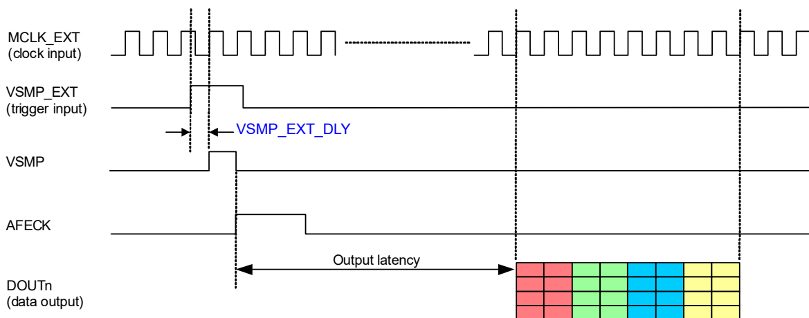
Figure 4-45. Data Output Timing (External Mode 2)
