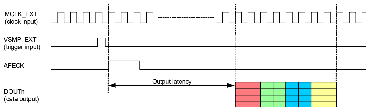
Figure 4-43. Data Output Timing (External Mode 1)
