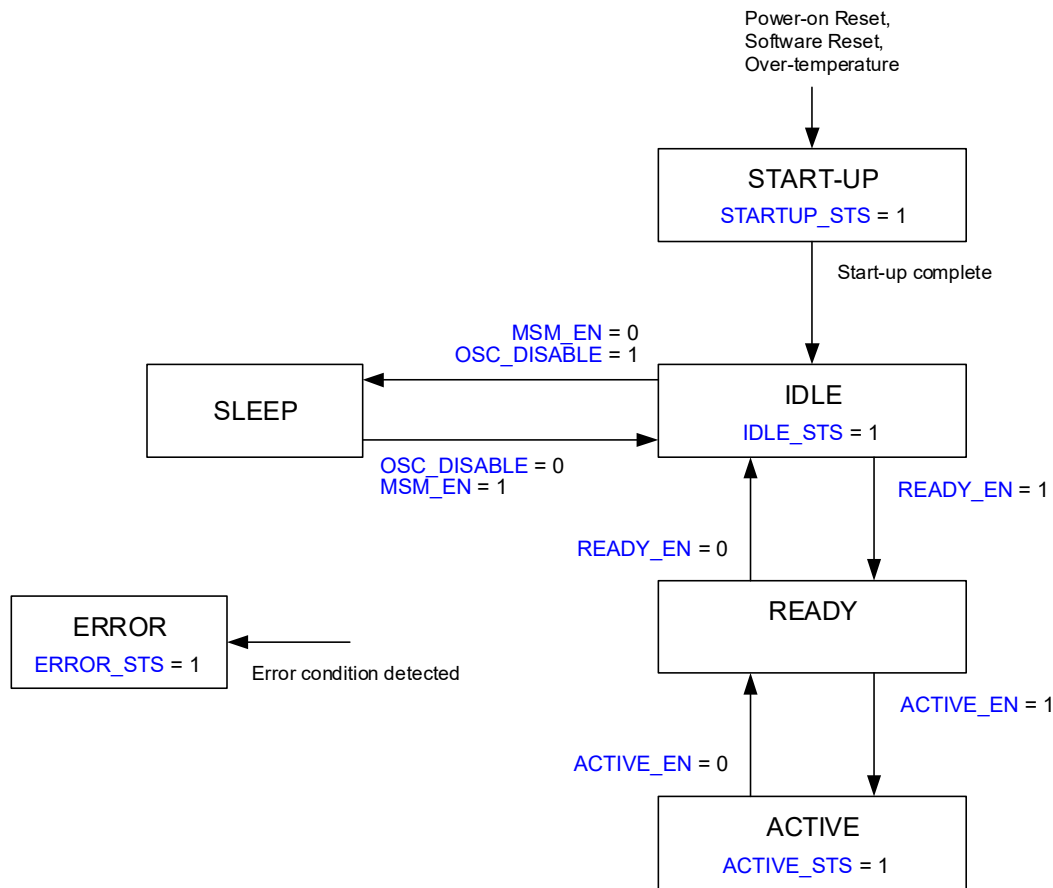
Figure 4-1. Operational States
