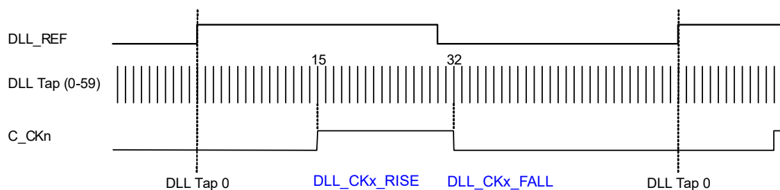
Figure 4-61. High-Speed Clocks (C_CKn)
