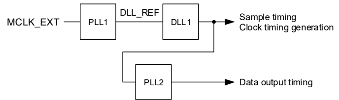
Figure 4-7. Clocking Mode 2
