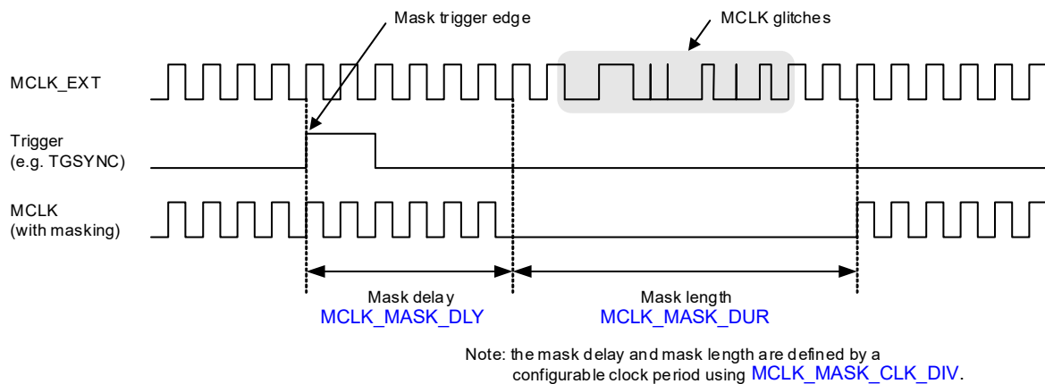
Figure 4-8. MCLK Masking
