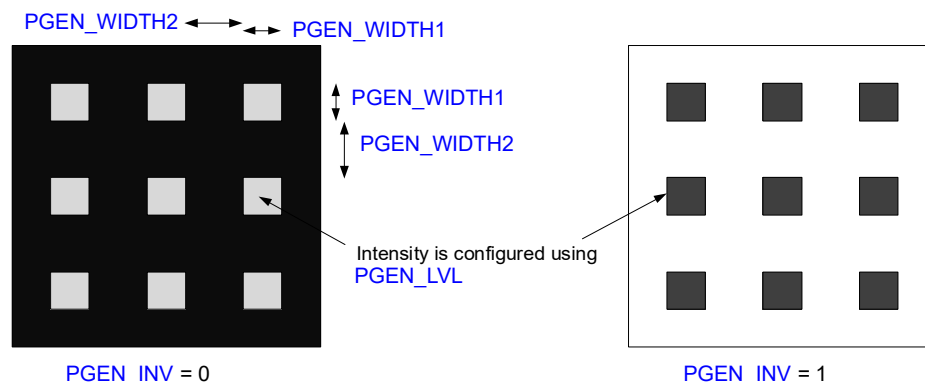
Figure 4-24. Patch Pattern
