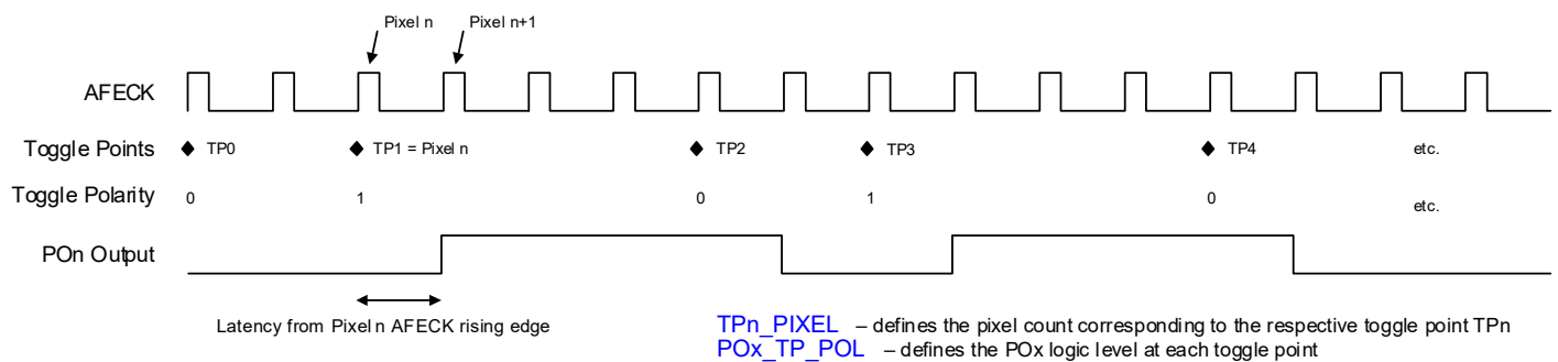
Figure 4-57. Pulse-Output (POn) Configuration—Toggle Point Control
