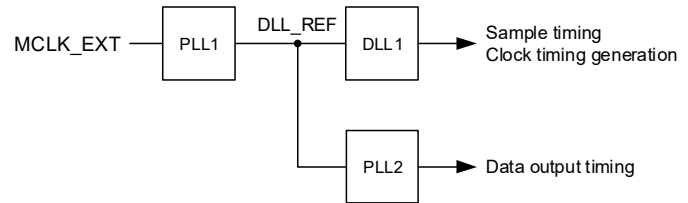
Figure 4-6. Clocking Mode 1
