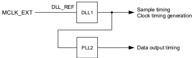
Figure 4-5. Clocking Mode 0
