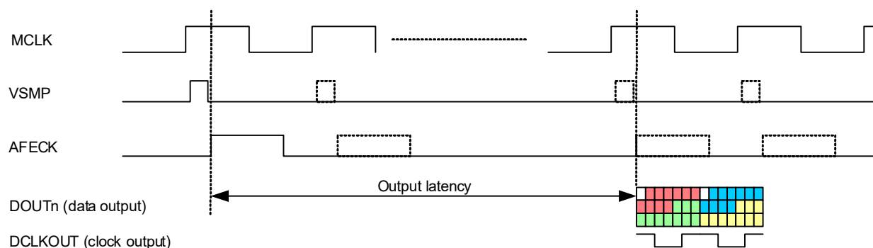
Figure 4-43. Data Output Timing (TG Mode, LVDS Output)
