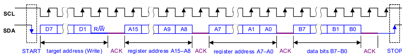
Figure 4-70. Control Interface I 2 C Register Write
