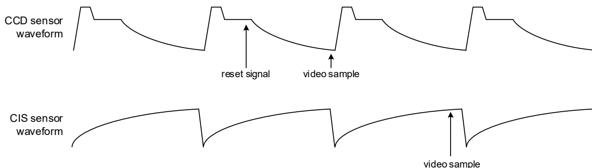
Figure 4-10. Typical CIS/CCD Waveforms
