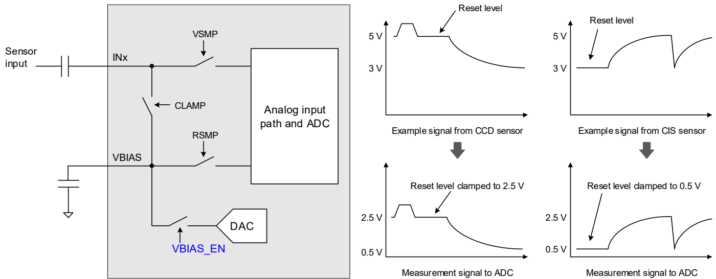
Figure 4-11. Input Clamp
