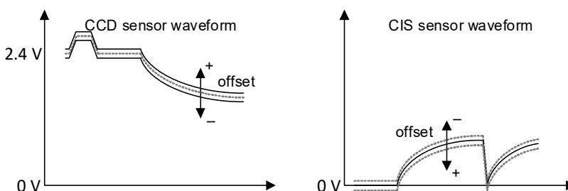
Figure 4-15. Offset Control
