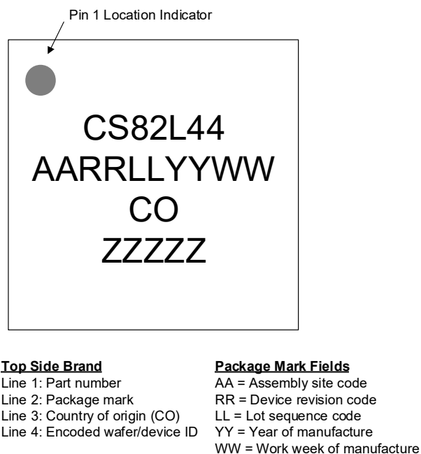
Figure 11-1. Package Marking
