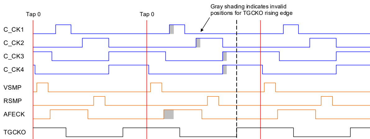
Figure 4-68. Example Clocking Configuration
