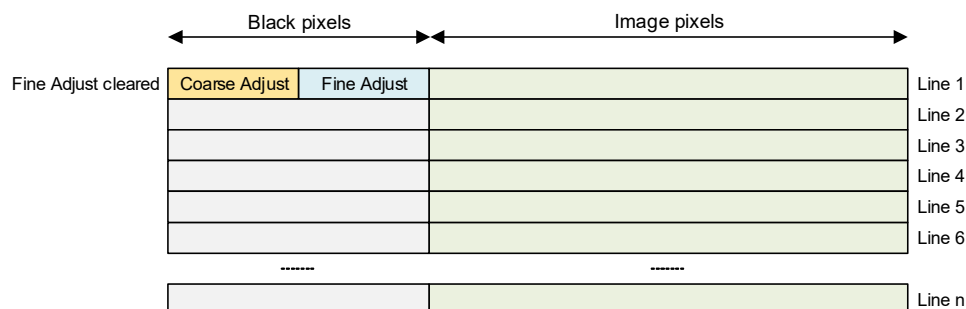
Figure 4-20. Black Level Calibration—Example 2
