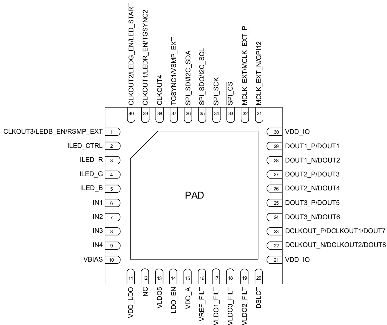
Figure 1-1. QFN 40-pin diagram (Top View, Through Package)
