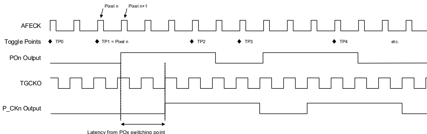
Figure 4-59. Pulse Clock (P_CK) Configuration
