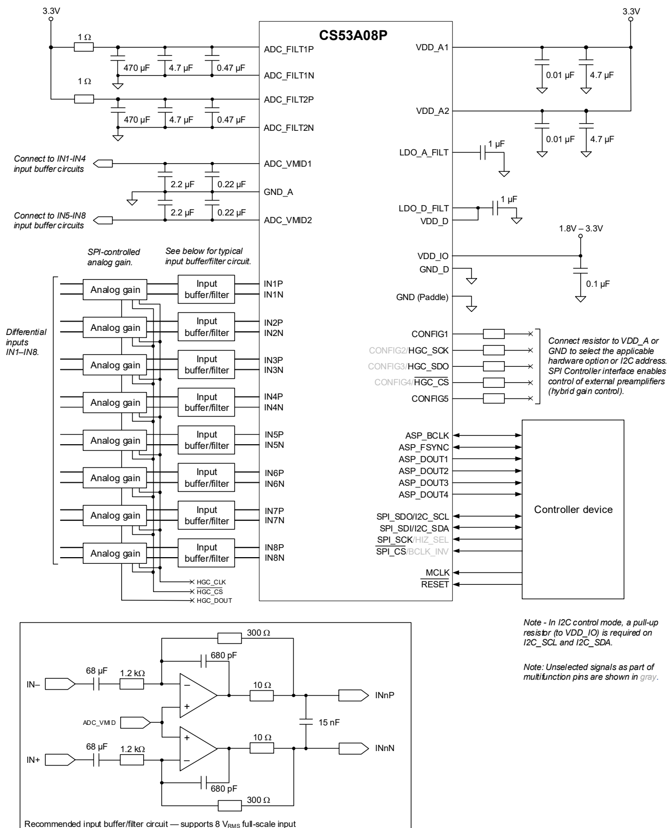
Figure 2-1. Typical Connections
