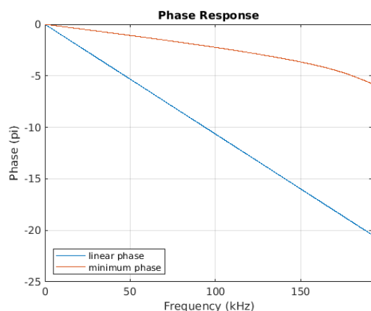
Figure 8-47. Phase vs. Frequency
