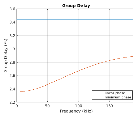
Figure 8-54. Group Delay vs. Frequency
