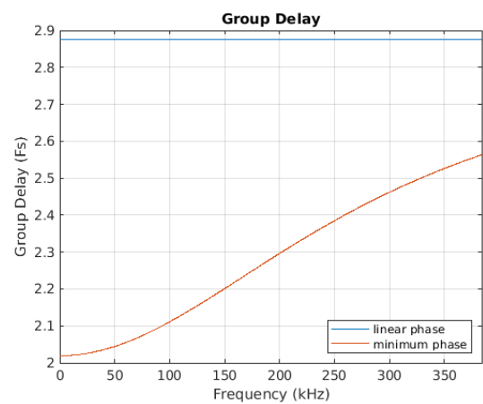
Figure 8-66. Group Delay vs. Frequency
