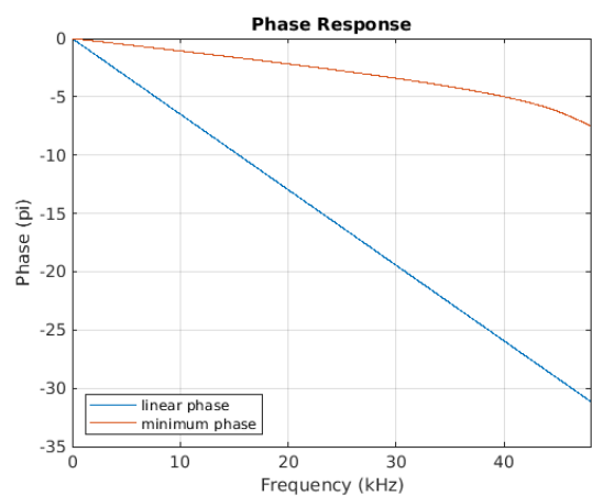
Figure 8-23. Phase vs. Frequency
