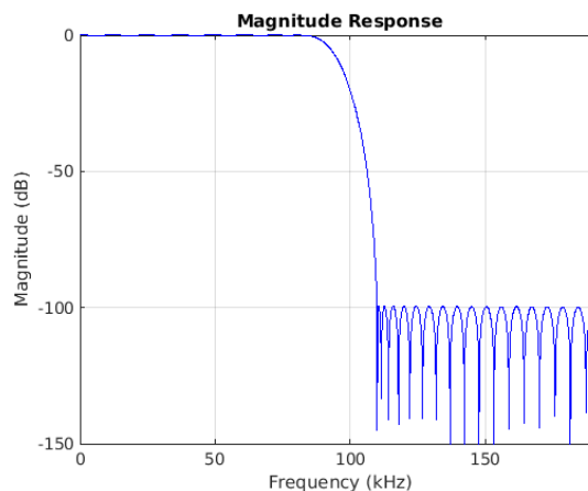
Figure 8-32. Stopband Magnitude
