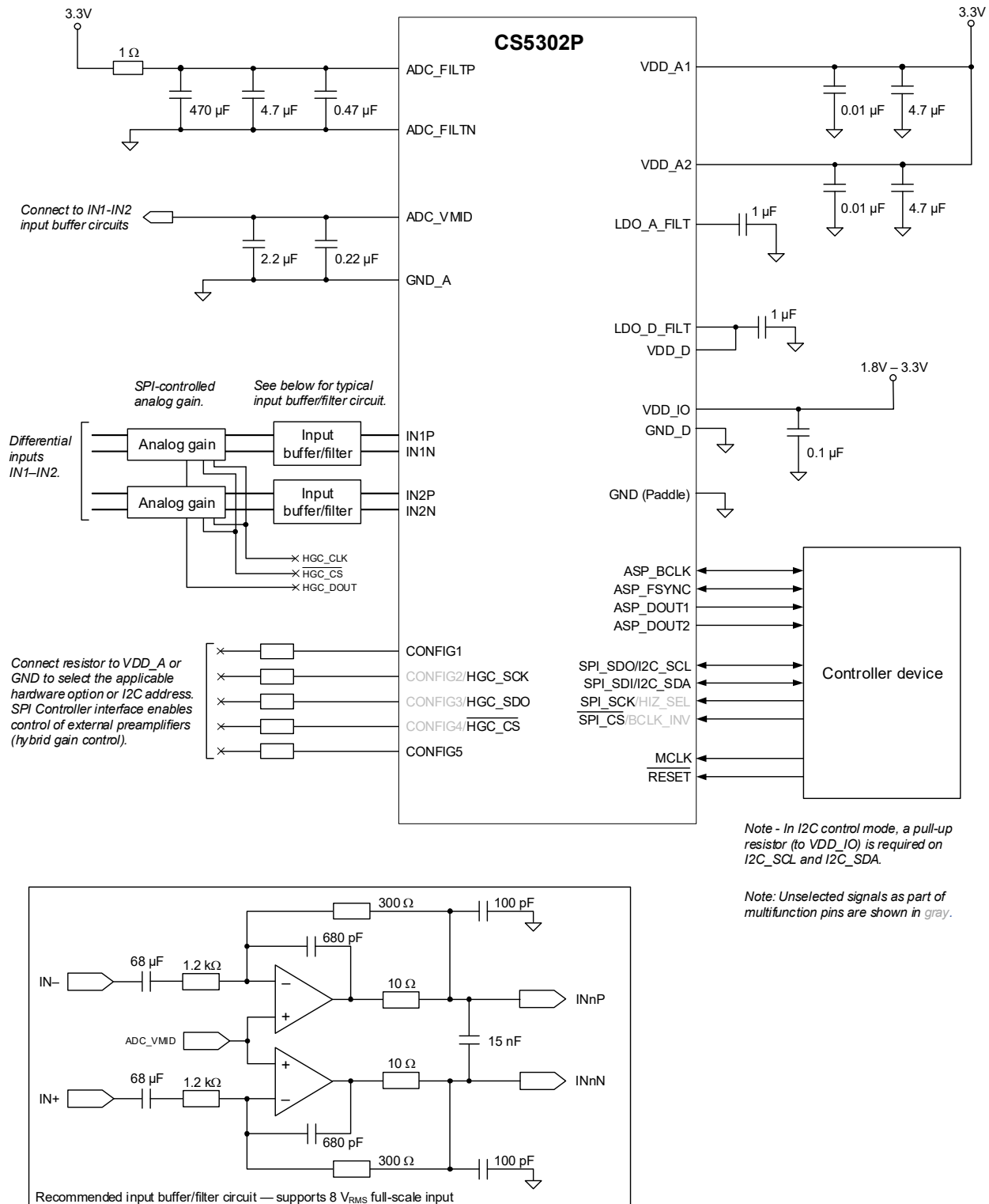
Figure 2-1. Typical Connections
