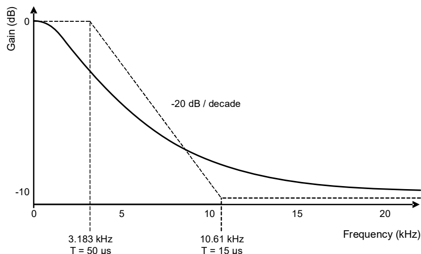
Figure 4-9. Deemphasis Filter Response
