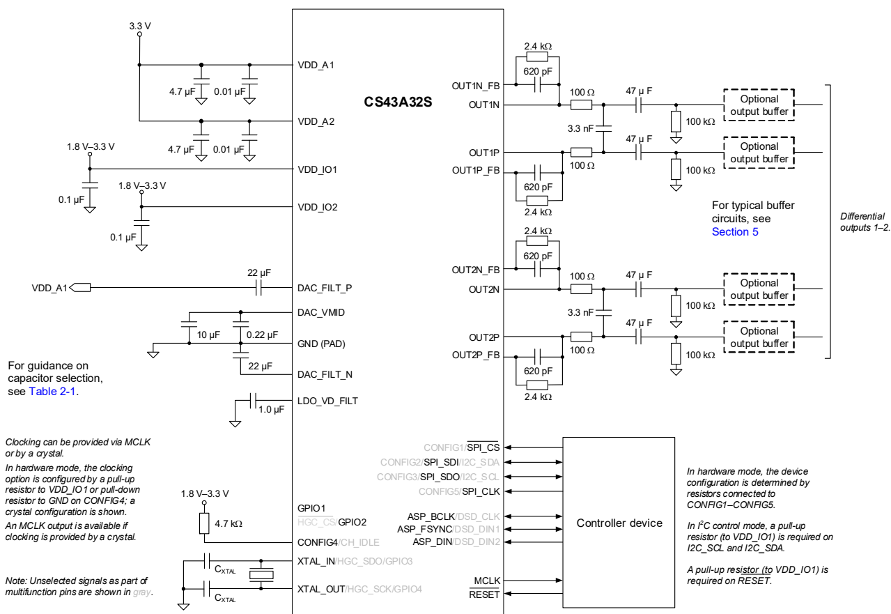
Figure 2-1. Typical Connections
