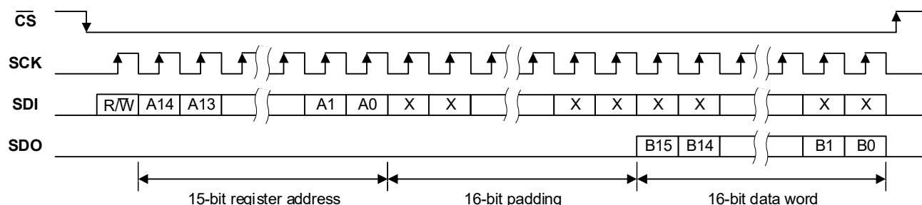
Figure 4-35. Control Interface SPI Register Read
