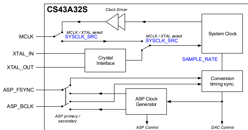
Figure 4-2. System Clocking
