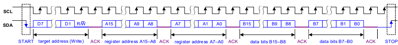
Figure 4-28. Control Interface I 2 C Register Write
