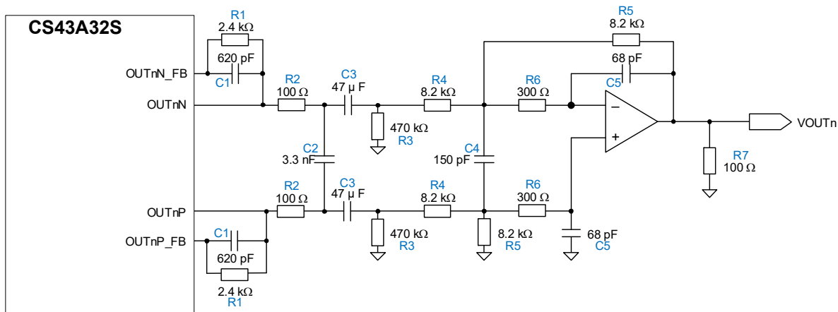
Figure 5-3. Example Differential-to-Single-Ended Output Circuit
