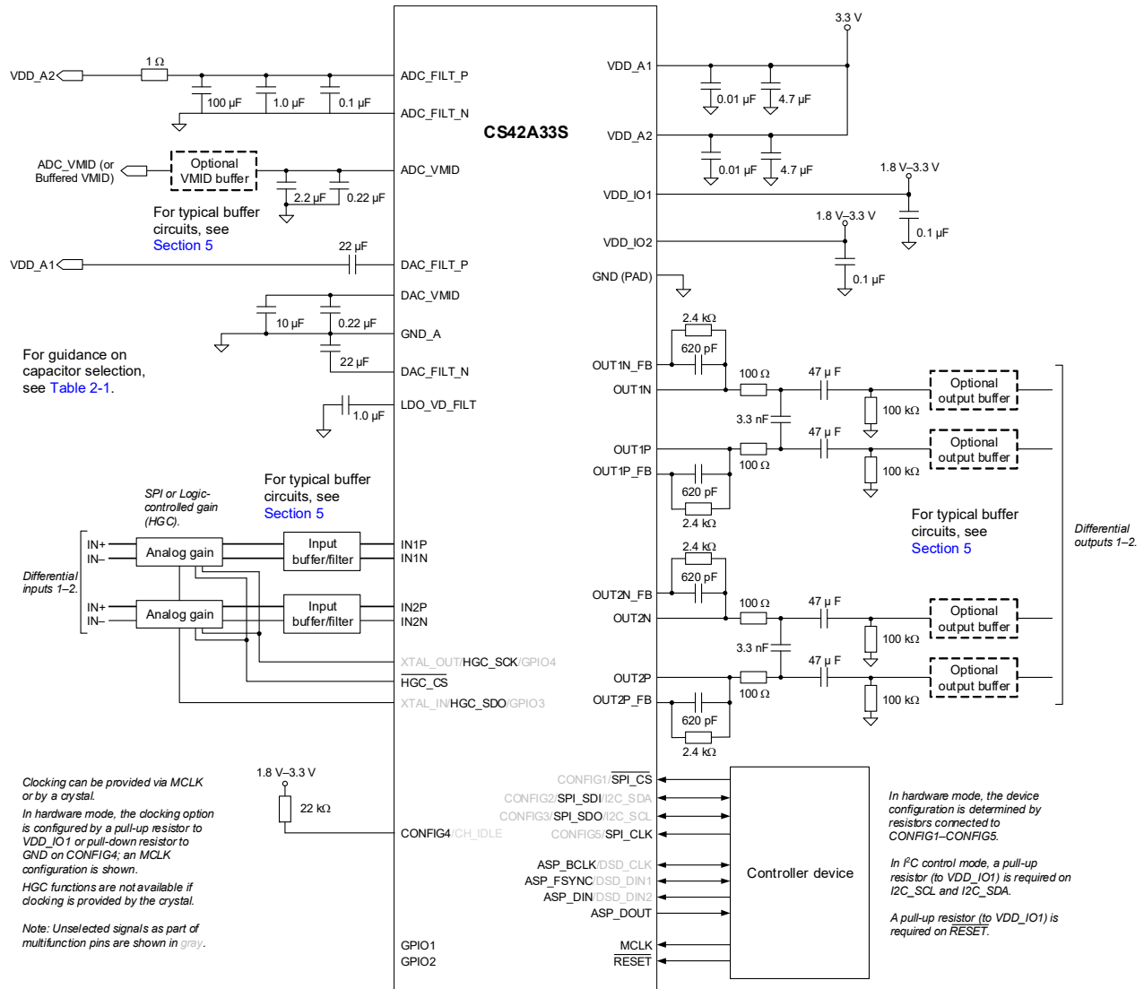
Figure 2-1. Typical Connections
