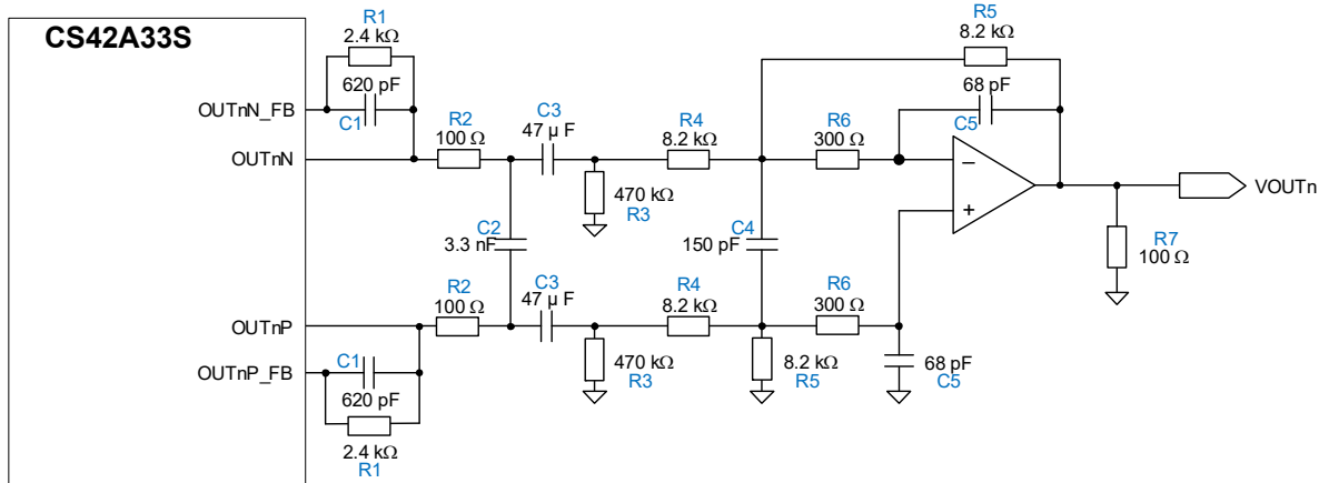
Figure 5-4. Example Differential-to-Single-Ended Output Circuit
