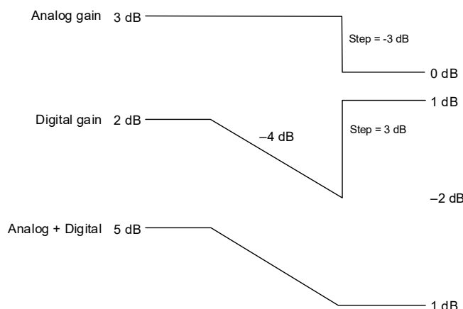
Figure 4-8. Output Path Negative Gain Ramping
