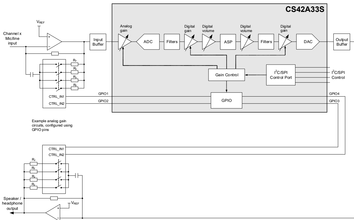
Figure 4-4. Hybrid Gain Control using GPIO Pins
