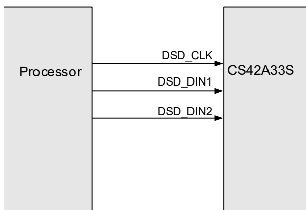
Figure 4-24. DSD Interface Connection
