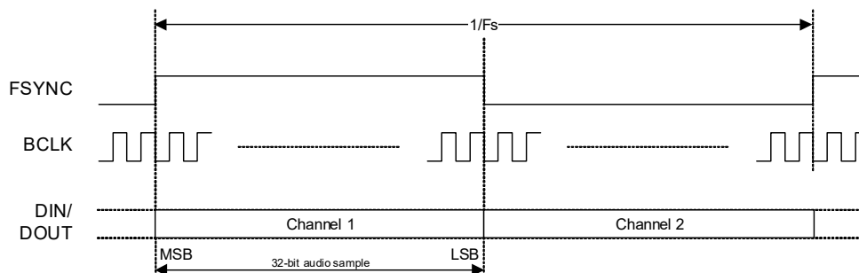
Figure 4-21. Left-Justified Data Format
