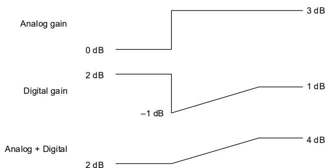
Figure 4-7. Input Path Positive Gain Ramping
