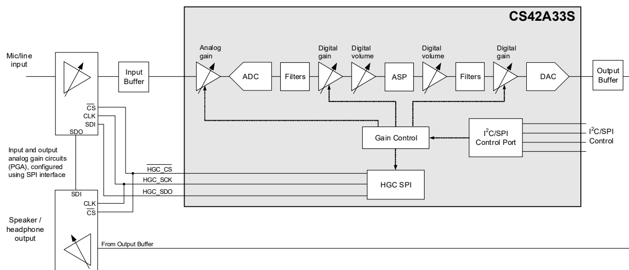
Figure 4-3. Hybrid Gain Control using HGC SPI
