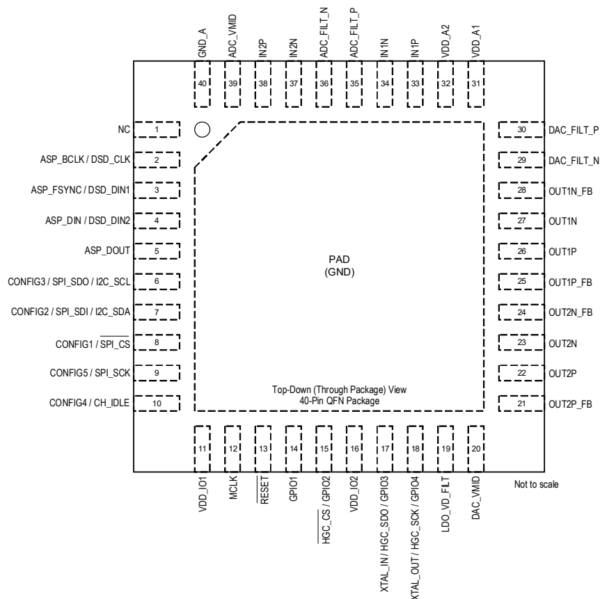
Figure 1-1. QFN 40-Pin Diagram (Top View, Through Package)
