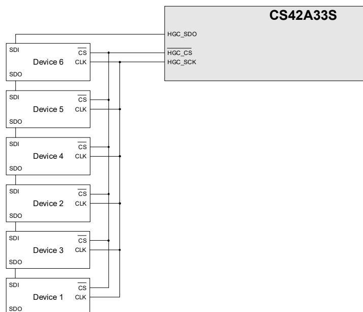
Figure 4-6. HGC SPI Daisy Chain Example Connections
