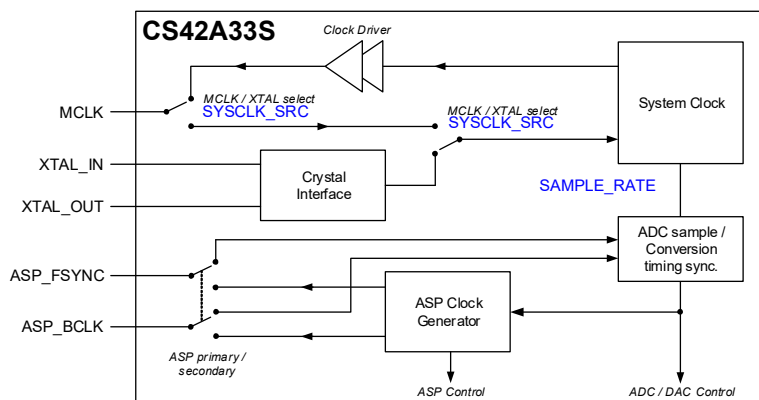
Figure 4-2. System Clocking
