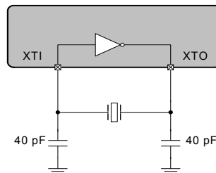
Figure 9. External Component Requirements for Crystal Circuit
