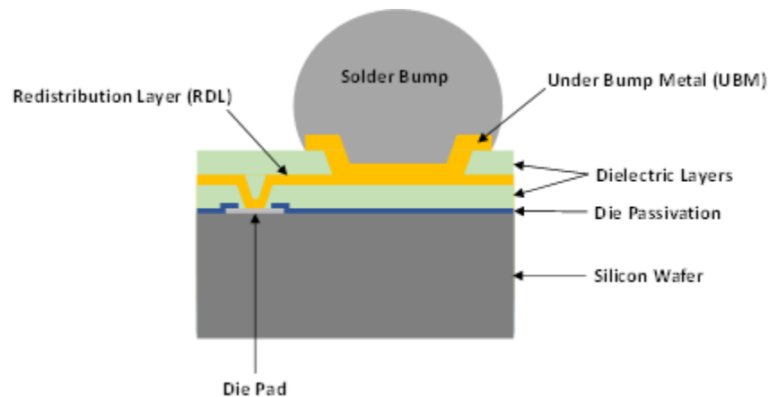
Figure 2: WLCSP Cross Section
