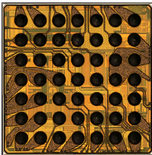
Figure 1: Typical WLCSP Device
