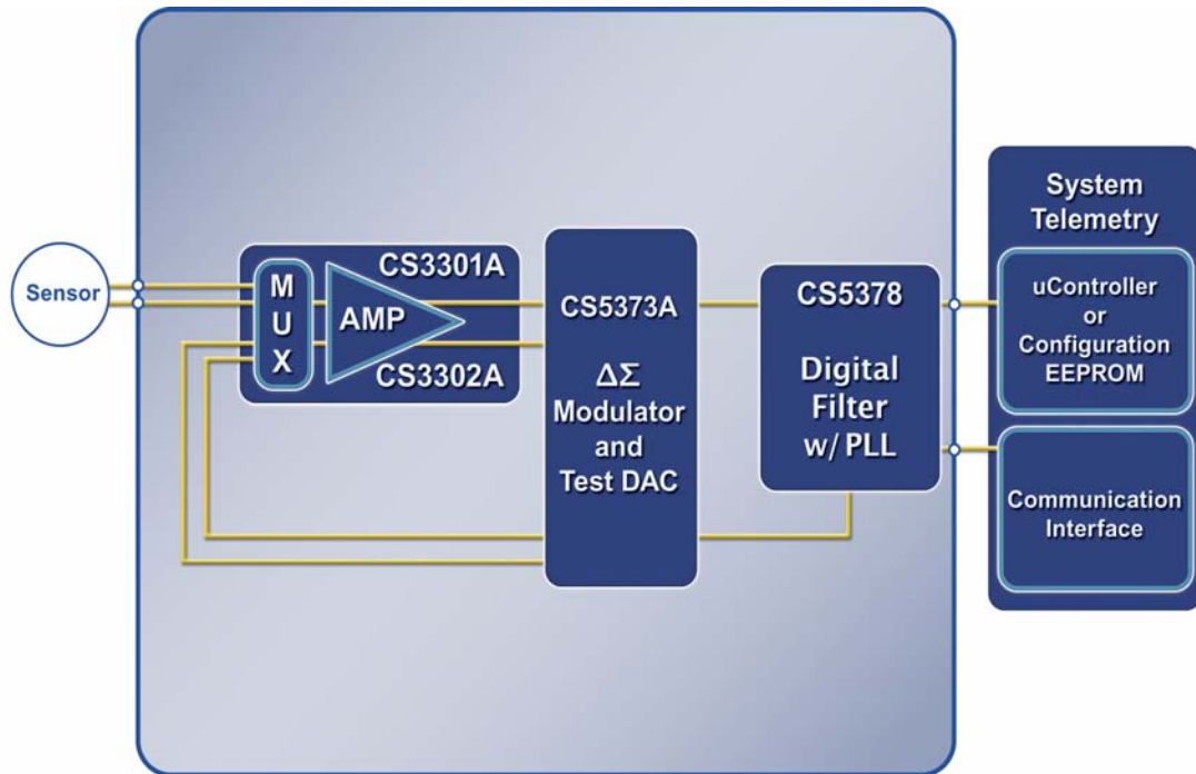
Figure 1. CDB5378 Block Diagram
