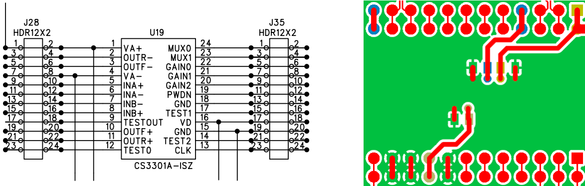
Figure 7. Dual-row Headers with Shorts
