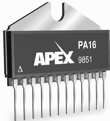
12-pin SIP PACKAGE STYLE DP Formed leads available See package style EE
