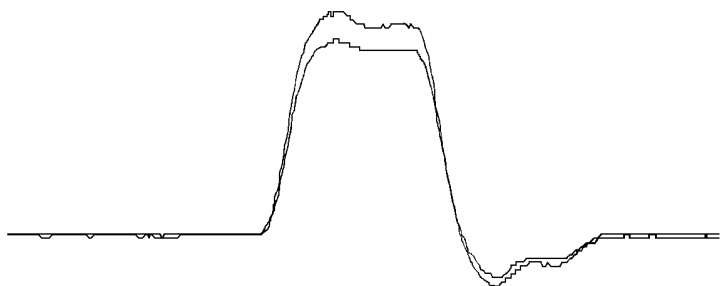
Figure 8 - Mismatch and gain error can have significant effect on pulse amplitude. The larger pulse results from the use of probes which are not well matched,
