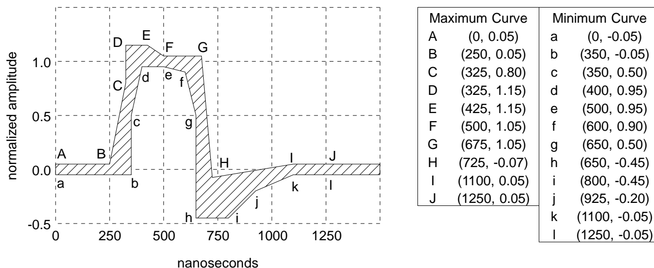
Figure 1. ANSI T1.102 - 1993 T1 pulse template
