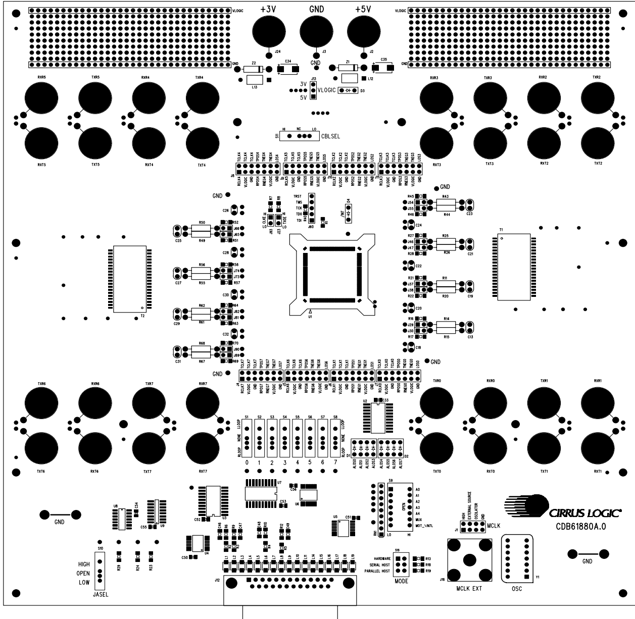
Figure 1. CDB61880 Board Layout
