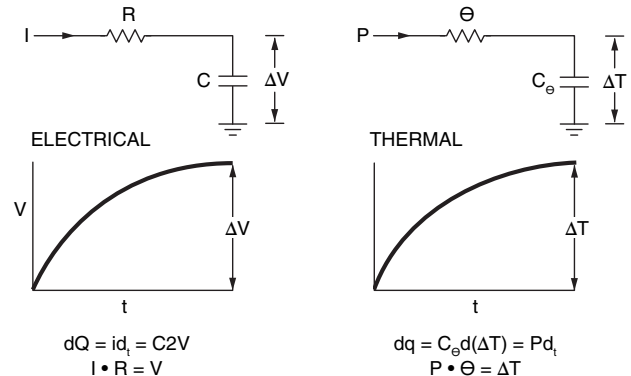
FIGURE 8. Electrical and Thermal Models.
